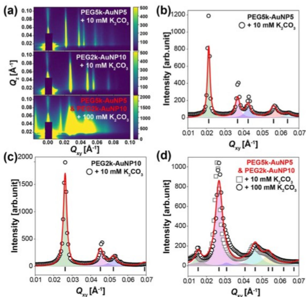
<Figure 3.2.6.8> (a) GISAXS patterns for AuNPs synthesized by different PEG conditions. (b)-(d) Line-cut intensity as a function of Q_{xy} . Reproduced from Ref Kim et al. , (2022) with permission.
