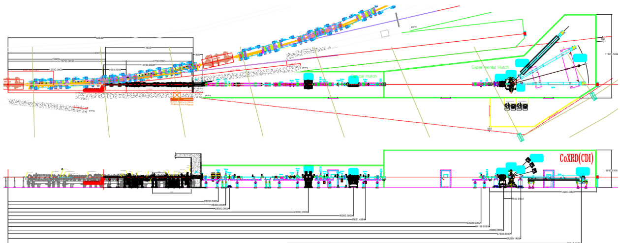
<Figure 3.2.5.2> Coherent X-ray Diffraction Beamline drawing.
