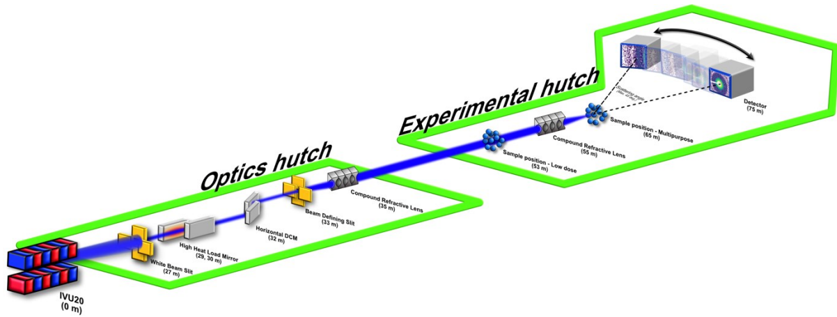
<Figure 3.2.6.11> The overview of the layout of COSAXS beamline.
