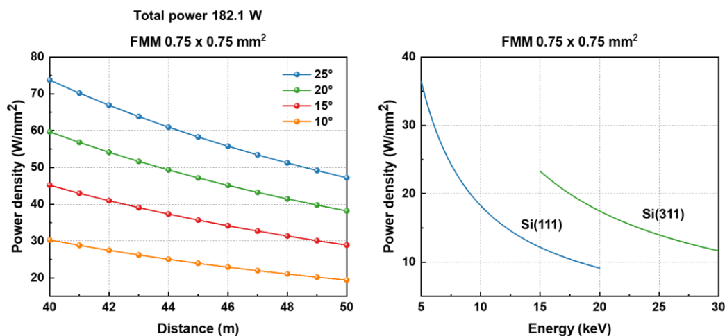
<Figure 3.2.5.8> Calculated power density on the HDCM with FMM opening of 0.75 x 0.75 mm 2 .
