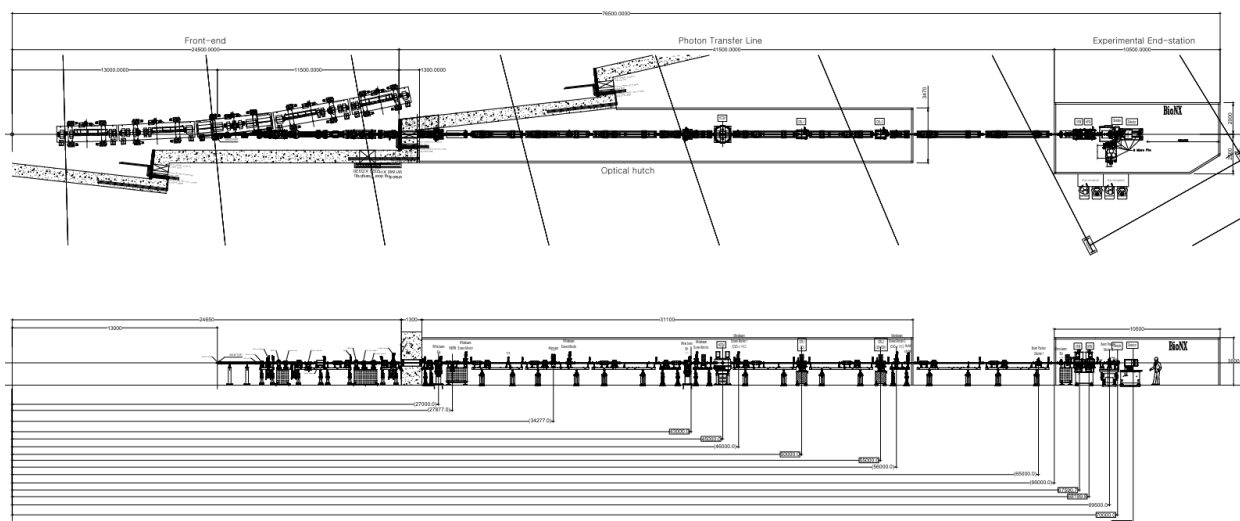
<Figure 3.2.8.3> Beamline layout of BioNX.
