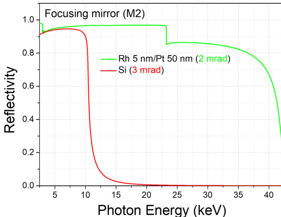
<Figure 3.2.7.9> Reflectivity curve of the HFM.
