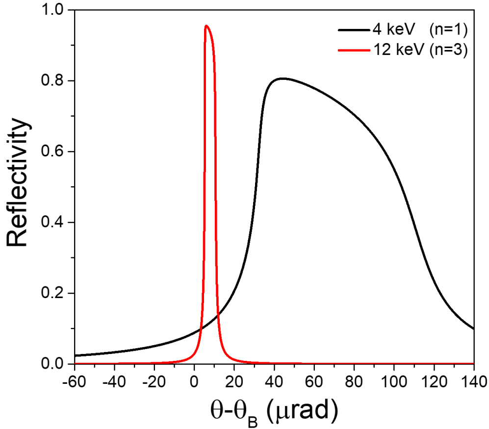
<Figure 3.2.7.8> Darwin width curve of Si(111).
