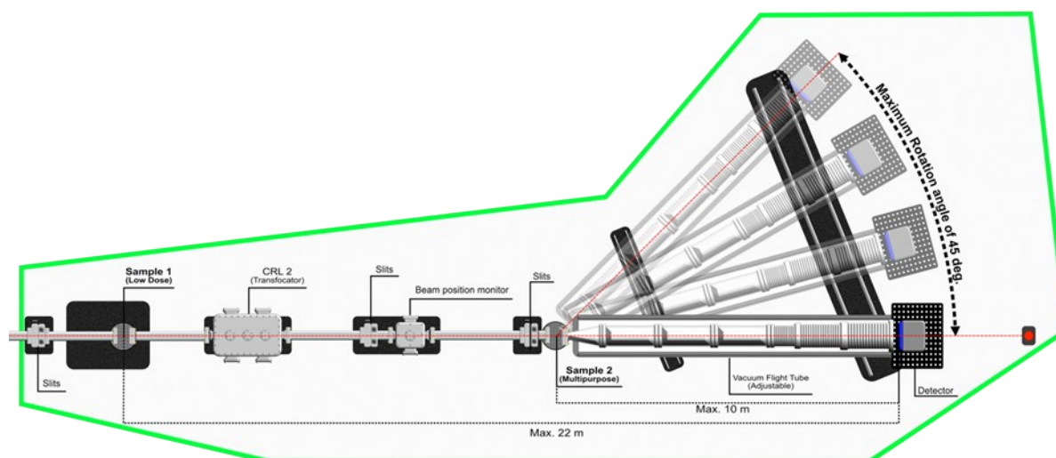
<Figure 3.2.6.16> Schematic of the experimental hutch of ID04.
