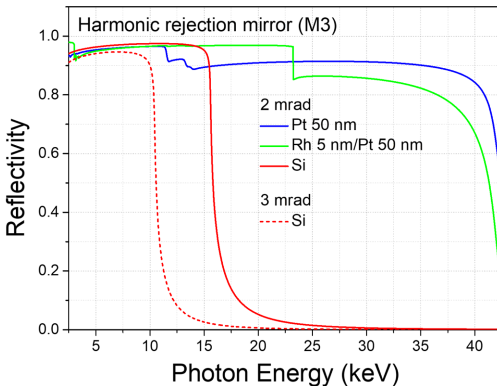
<Figure 3.2.7.10> Reflectivity curve of HRM.
