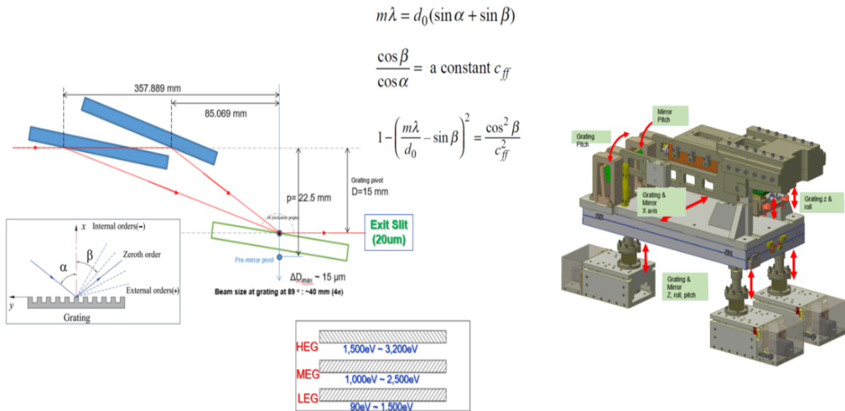
<Figure 3.2.3.12> Monochromator Internal Schematic.
