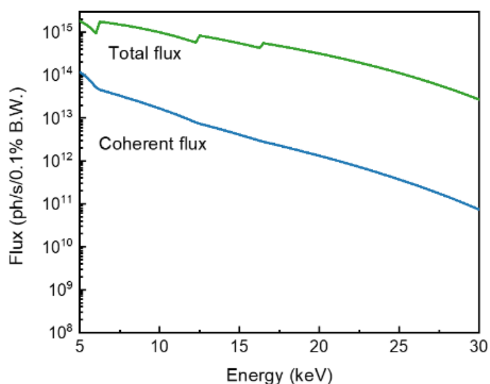
<Figure 3.2.5.5> IVU22 source total flux and coherent flux at 5-30 keV(0.1% B.W.).
