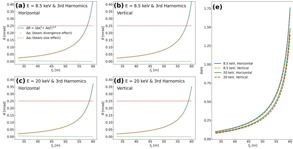
<Figure 3.2.6.14> Angle and wavevector resolutions as a function of position of focusing optics from the source f_p . The red dashed lines in (a)-(d) represent the \theta_{min} defined by the beam stop size.
