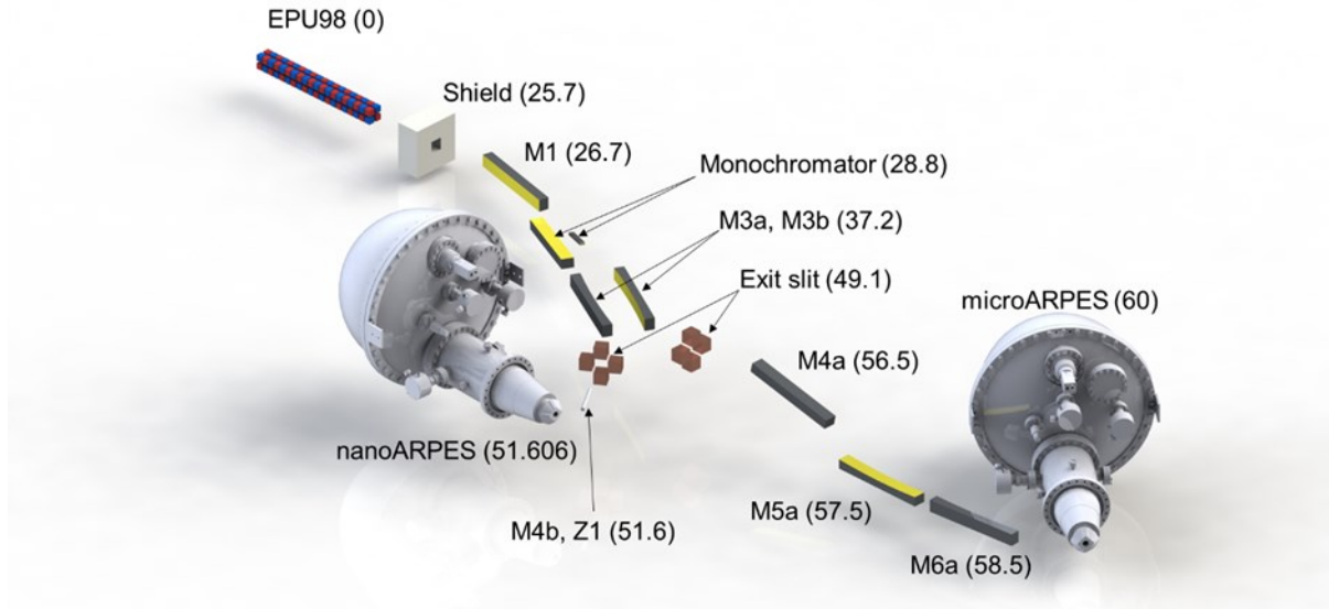
<Figure 3.2.4.3> Schematic overview of the nanoARPES beamline, including microARPES and nanoARPES branches.
