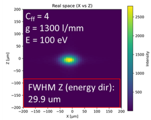
Single energy spot size at exit slit
