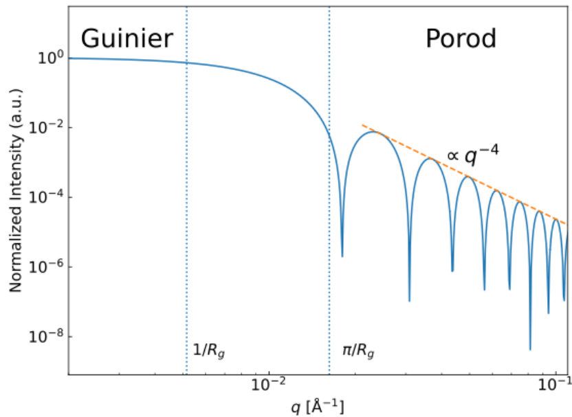
<Figure 3.2.6.7> Normalized SAXS curves of sphere with the radius of R = 25 nm.
