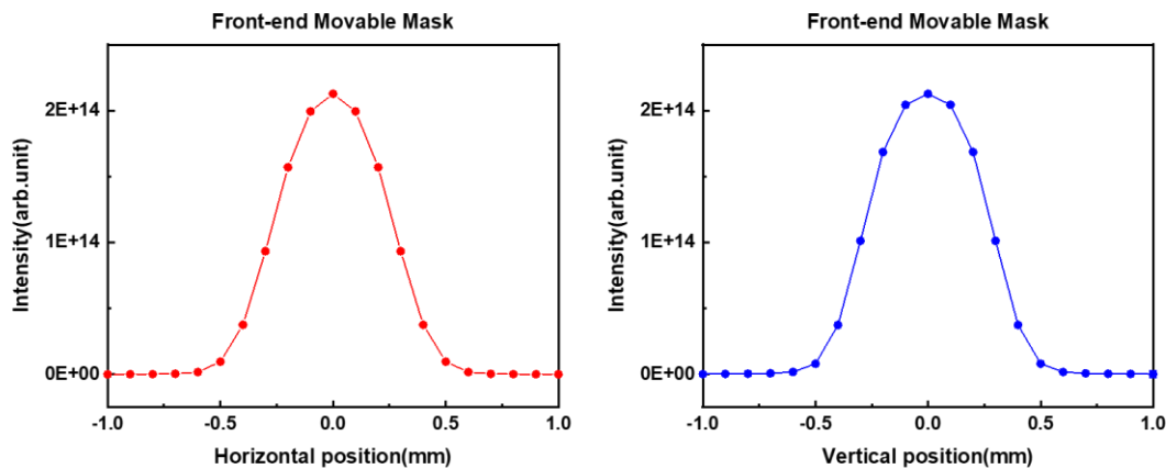
<Figure 3.2.5.10> Front-end Movable Mask alignment beam profile.
