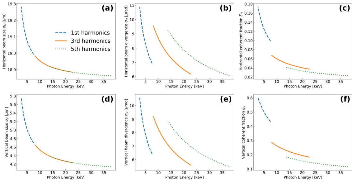
<Figure 3.2.6.10> Photon parameters of IVU20 estimated by SPECTRA.
