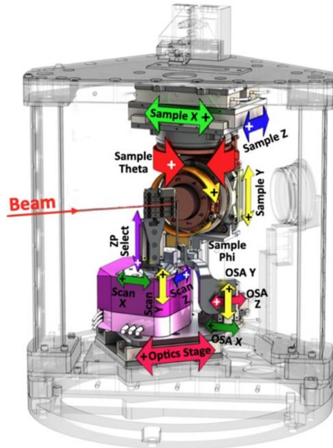
<Figure 3.2.4.14> nanoARPES sample stage at the MAESTRO.
