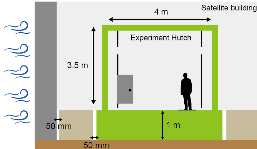
<Figure 3.2.10.11> Satellite building and hutch structure of Nanoprobe beamline.
