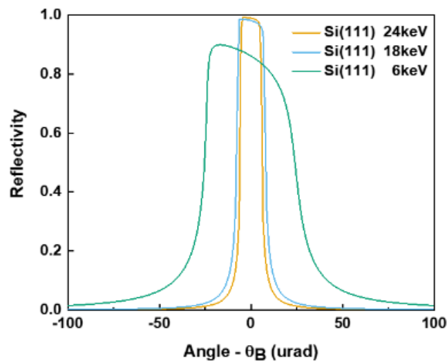
<Figure 3.2.5.11> Darwin width curve at 6 keV and its high-order harmonics.
