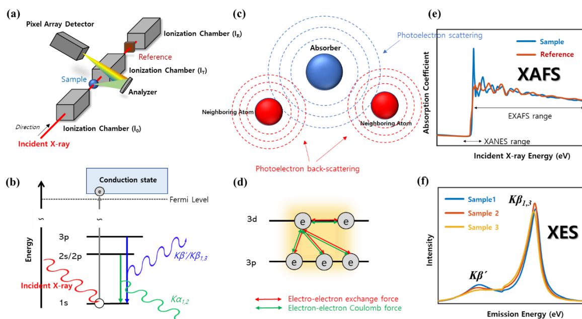
<Figure 3.2.7.21> (a) Schematic diagram of simultaneous XAFS and XES measurements. A monochromatic beam excites the electrons in atoms, and both transmitted and emitted signals are collected. (b) Schematic of atomic energy levels showing excitation and emission process. (c) Principle of XAFS: A photoelectron excited by the incident X-ray is backscattered by neighboring atoms. This interference modulates the absorption coefficient, allowing the analysis of local environment. (d) Principle of XES: Electronic interactions, such as exchange and Coulomb forces surrounding electrons, cause shifts in fluorescence energy (e) Example of XAFS spectra showing both XANES and EXAFS regions for sample and reference (f) Example of XES spectra showing the variation in emission features for different samples.
