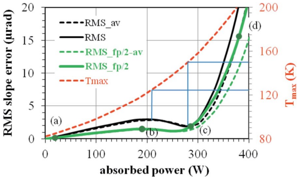
<Figure 3.2.6.18> RMS thermal slope error and the maximum temperature of the ID06 LN2-cooled silicon crystal as a function of absorbed power. 52
