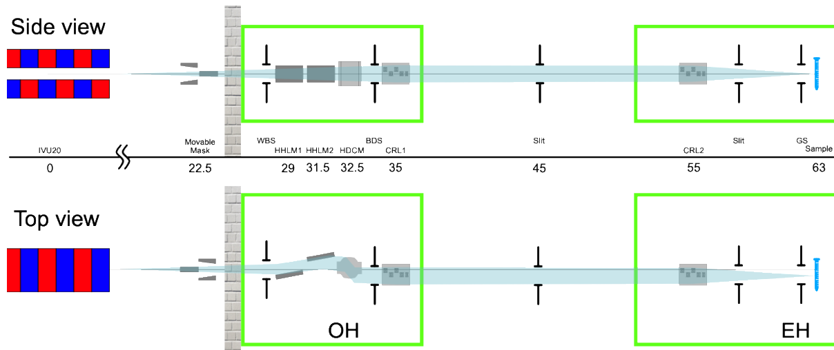
<Figure 3.2.6.16> The optical layout of COSAXS beamline when the beam is focused on the multipurpose sample position for XPCS.
