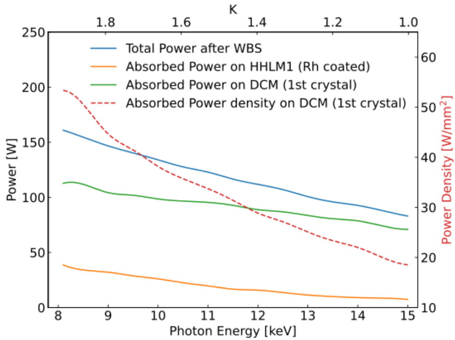
<Figure 3.2.6.19> Heat load calculation on the HHLM and DCM as a function of photon energy and K.
