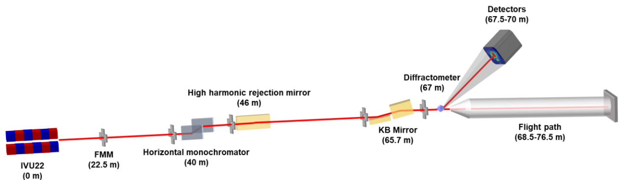
<Figure 3.2.5.5> Coherent X-ray Diffraction Beamline layout schematic.
