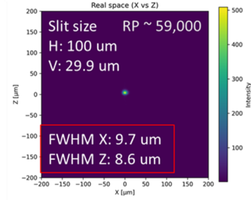
Single energy spot size at uA focus
