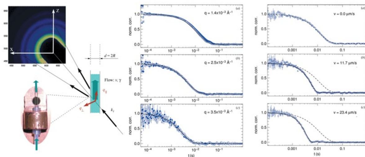
<Figure 3.2.6.18> XPCS measurement at a microfluidic system. The flow effect on the dynamics was decoupled by the dedicated data analysis.
