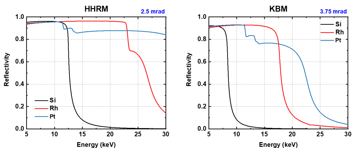
<Figure 3.2.5.9> Reflectivity of the HHRM(2.5 mrad) and KBM(3.75 mrad) as a coating materials.
