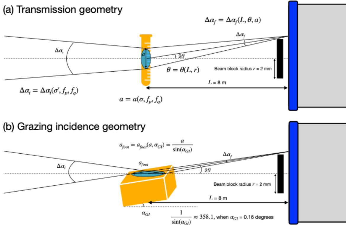
<Figure 3.2.6.13> Schematic of (a) conventional SAXS and (b) Grazing incidence SAXS geometry.
