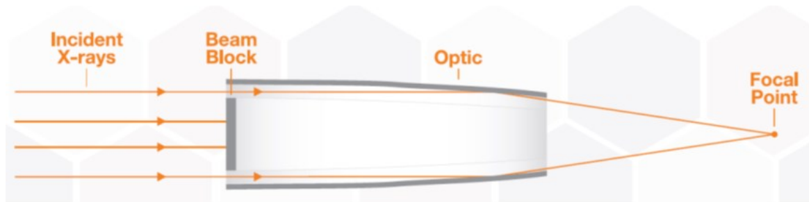
<Figure 3.2.4.13> The cross-section of a capillary mirror, including central beam stop to block the unfocused portion of the beam.
