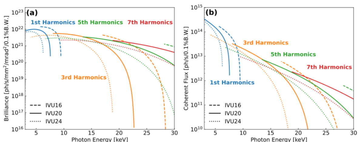
<Figure 3.1.1> Photon brilliance and coherence flux for IVU16, IVU20 and IVU24.
