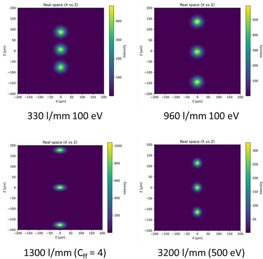
<Figure 3.2.4.9> Ray tracing result at the exit slit, with energy of 100 (500) eV and 100 (500) \pm 0.01 (0.05) eV, resolving power = 10,000. The intensity is shown in arbitrary units.
