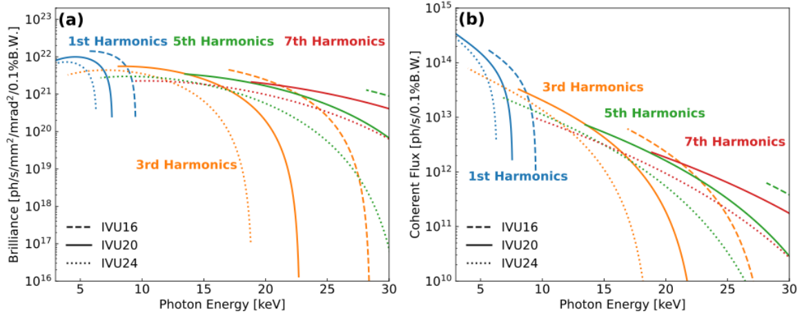
<Figure 3.2.6.9> Estimated X-ray beam parameters for three undulator periods, e.g., \lambda_u of 16, 20, and 24 mm are represented by dashed, solid, and dotted lines, respectively.
