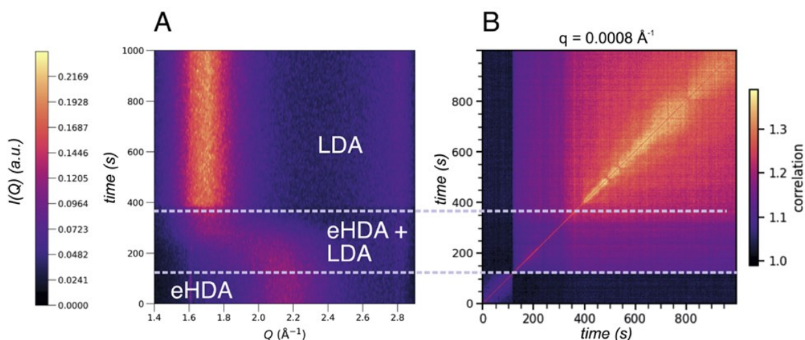
<Figure 3.2.6.19> (a) X-ray scattering signals from low- and high-density amorphous ices at WAXS regime, and (b) the XPCS result at SAXS regime.
