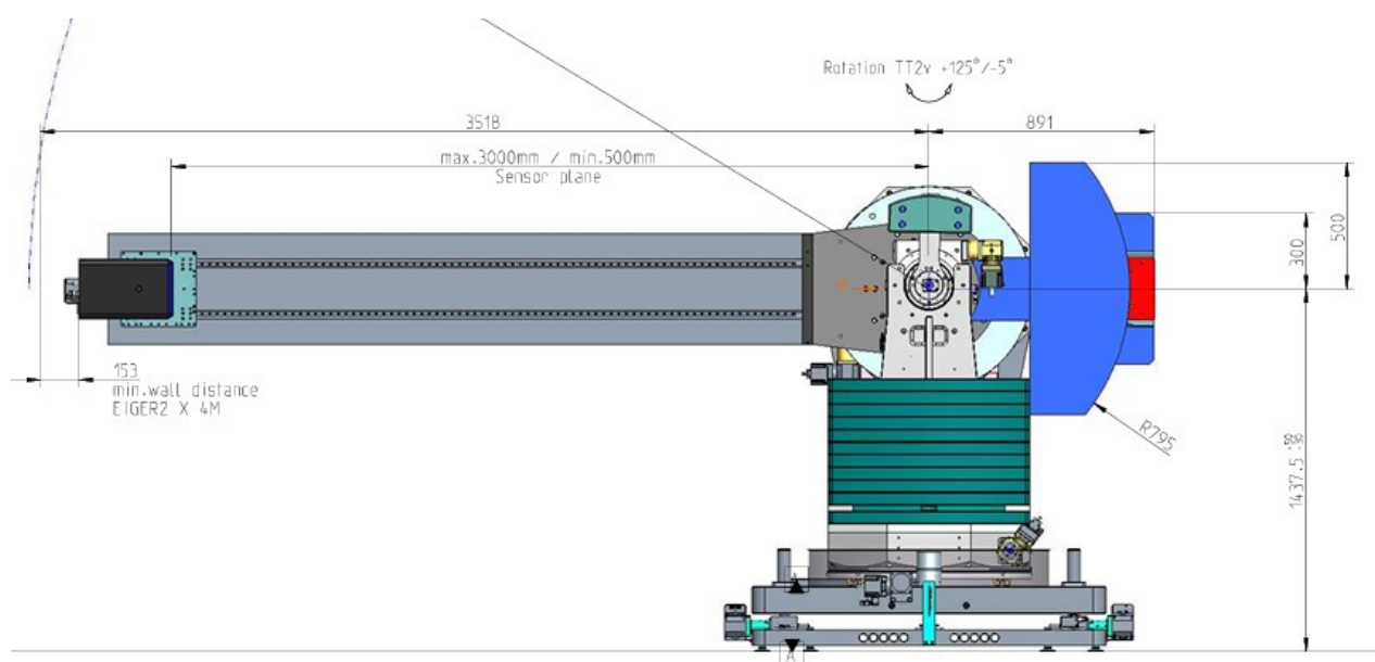
<Figure 3.2.5.13> Design of the 6-circle diffractometer with Kappa goniometer.
