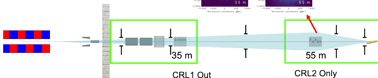
<Figure 3.2.6.20> Focusing schemes for transmission SAXS (upper) and grazing incidence SAXS (lower) experiments. In the conventional SAXS configuration, the beam size at the CRL1 translocator is approximately 700 \mu\text{m} in both the horizontal and vertical directions. For the GISAXS configuration, the beam size is around 1000 \mu\text{m} in both directions.
