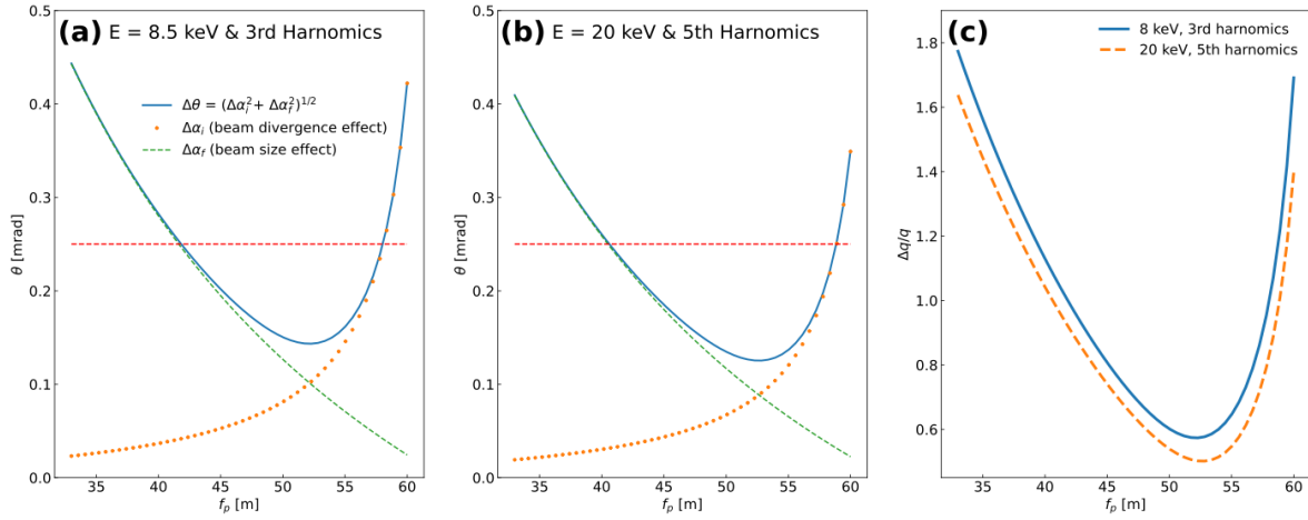
<Figure 3.2.6.15> Angle and wavevector resolutions as a function of position of focusing optics from the source f_p in vertical scattering directions.
