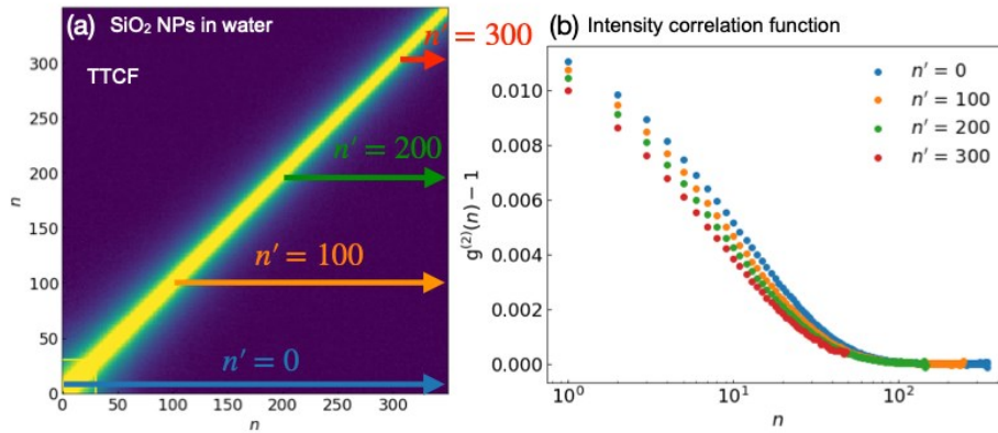
<Figure 3.2.6.6> XPCS result measured from European XFEL. (a) Two-time correlation function, and (b) extracted intensity correlation function for various number of X-ray pulses took into the calculation.
