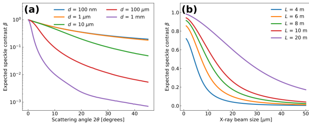
<Figure 3.2.6.12> Estimated speckle contrast \beta (a) as a function of scattering angle for various sample thickness and (b) as a function of X-ray beam size for various sample to detector distance.
