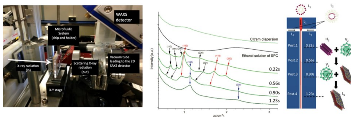
<Figure 3.2.6.17> Microfluidic system implemented at a synchrotron beamline. The X-ray scattering was obtained as a function of sample synthesis time.
