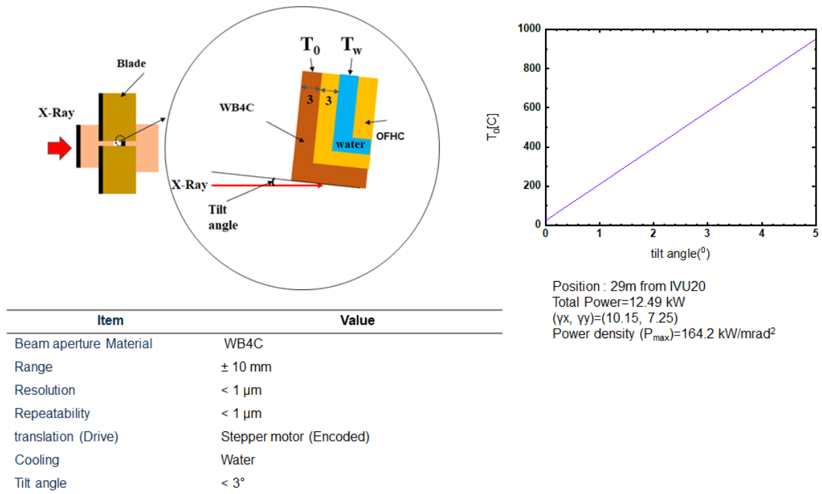
<Figure 3.2.6.17> The schematic structure of a typical slit and basic specifications.
